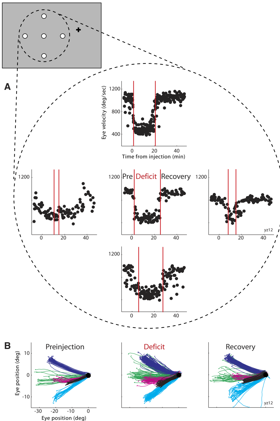
FIG. 1. Example of saccade changes during superior colliculus (SC) inactivation. A : saccade velocities show that the SC deficit field overlaps the frontal eye field (FEF) visuomovement field. Top left inset : the visuomovement field (dotted circle) of the FEF neuron in this experiment, which had presaccadic activity for saccades made from central fixation (crosshair) to each of 5 possible target locations (white circles). For this experiment, the center target was 5^\circ below and 20^\circ to the left of fixation. The other targets were 10^\circ from the center target. The expanded view (large dotted circle) shows the peak eye velocity in degrees per second (y axis) for saccades to each target, plotted as a function of time (x axis). Time zero indicates the beginning of the lidocaine injection. Red lines indicate the beginning and end of the deficit period for each location (see METHODS). For this experiment, eye velocities were significantly lower during the deficit period than during the preinjection period at all target locations, and the center location was chosen for neuronal analysis due to its strongest presaccadic activity. B : eye movement trajectories from the same example experiment show that the monkey can still make saccades. Trajectories for all locations are shown for the three analysis periods: preinjection, deficit, and recovery. x and y axes represent the horizontal and vertical eye positions in degrees of visual angle.
