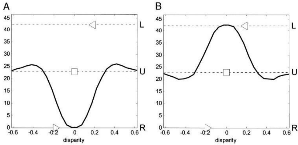
FIG. 4. Our new model, incorporating a threshold linearity before binocular combination, can explain disparity selectivity in classically monocular cells, and cells in which the response to binocularly uncorrelated dots ( U □) is close to the mean of response to monocular stimuli ( L ◀, R ▶), rather than to its sum as predicted by energy model. Both plots show simulations for single binocular subunit receiving inhibitory input from right eye (Eq. 5); mean response over 100,000 different random-dot patterns. A : monocular receptive fields are identical, so the inhibitory synapse in Eq. 5 results in a tuned-inhibitory cell. B : left eye’s receptive field is inverse of right eye’s receptive field, so with the inhibitory synapse this results in a tuned-excitatory cell.
