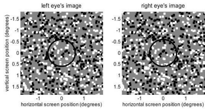
FIG. 2. Random-dot stereogram of type used in our experiments. Dots are 0.1^\circ \times 0.1^\circ square. Circle indicates size of typical V1 receptive field for comparison. Diameter is 1.2^\circ , based on a subset of cells in which we obtained the one-dimensional receptive field envelope using a long luminance-modulating bar stimulus at the preferred orientation. The mean SD of Gaussians fitted to receptive field envelopes was 0.3^\circ , and we took 4 SDs as suitable estimate of receptive field diameter.
